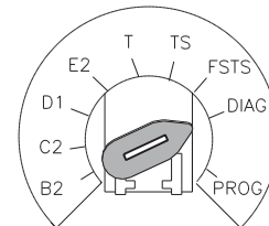
SELECTOR DIAL
